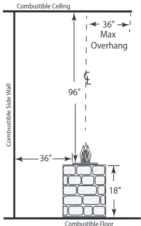
Fig. 3 Clearance to Combustibles (Not to be used in an enclosed space)
